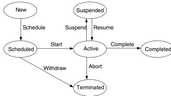
Fig. 5. A FSM describing the event types.
